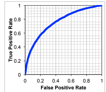
Figure 1. ROC curve for the TagCtCoCap model.
